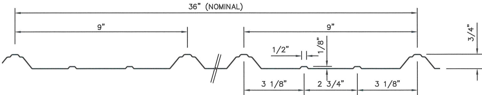
PANEL PROFILE
